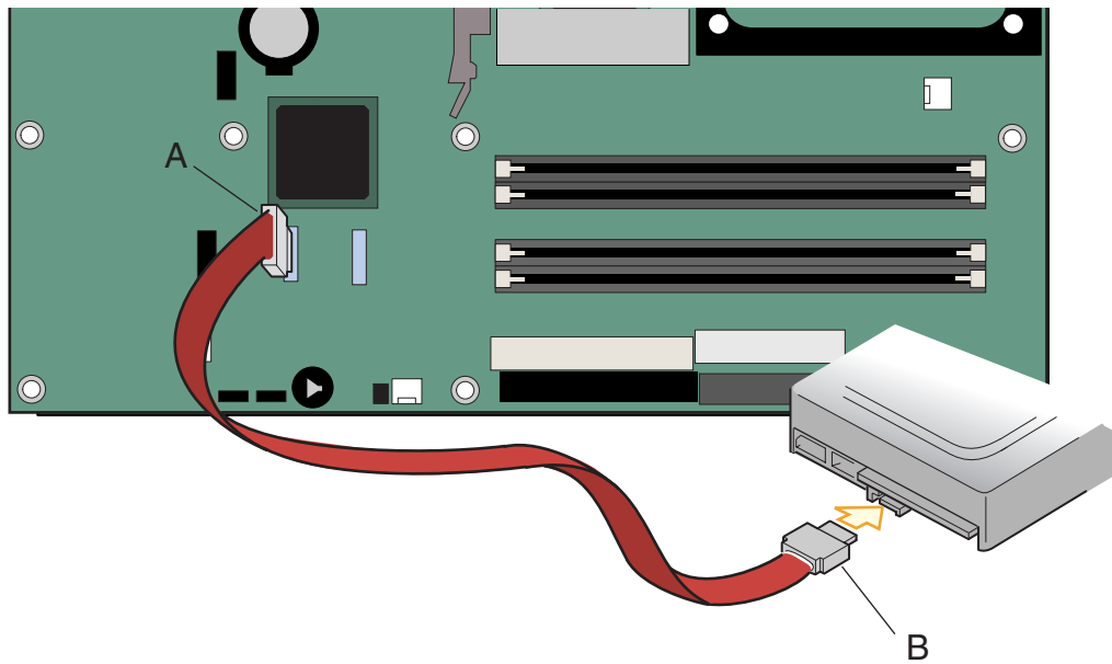
Figure 12. Connecting the Serial ATA Cable
